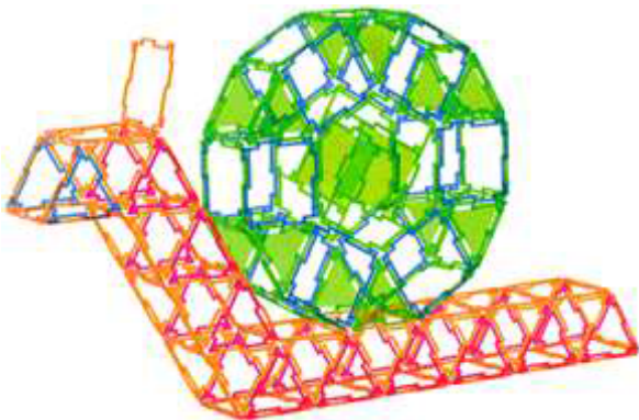
Built using 50 small equilateral triangles, 45 squares and 2 hexagons with square
