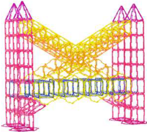
Built using 23 small equilateral triangles, 1 64 squares, 12 hexagons with square and 16 isosceles triangles
