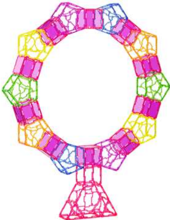
Built using 8 small equilateral triangles, 80 squares, 20 pentagons with triangle and 2 hexagons
